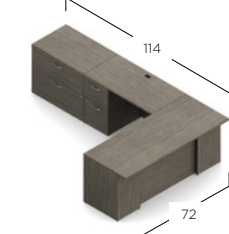
LAYOUT ZIRA MANAGER2 Z3072F3R+HQ Z16L2ES+HQ Z2448EL Z36L2E+HQ $3945
